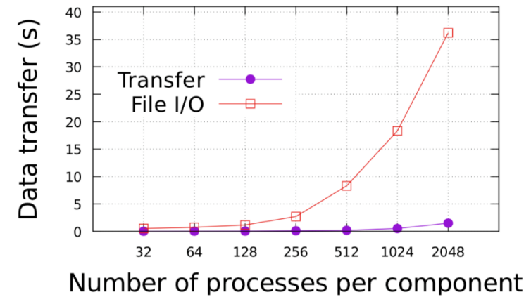
S3D-IO data transfer benchmark
