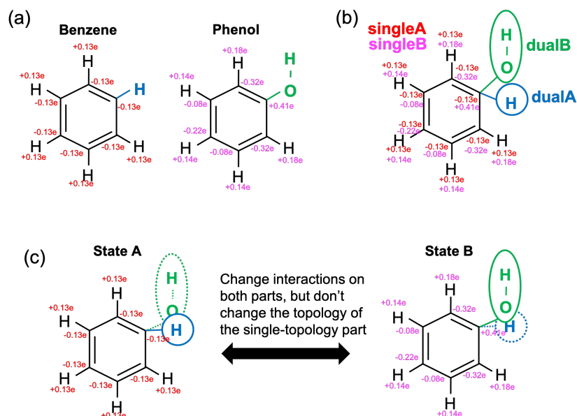
Fig. 21.3: Hybrid topology approach. (a) Benzene and phenol. H atom of benzene and OH atoms of phenol are in cyan and green, respectively. The point charges on common atoms are shown in red and magenta, which are determined using Amber Tools. (b) Hybrid topology of benzene and phenol. (c) The alchemical transformation from benzene to phenol.
